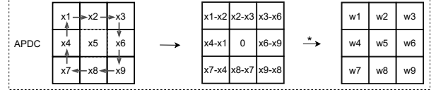
Figure 11. Selection of pixel pairs and convolution in APDC.
