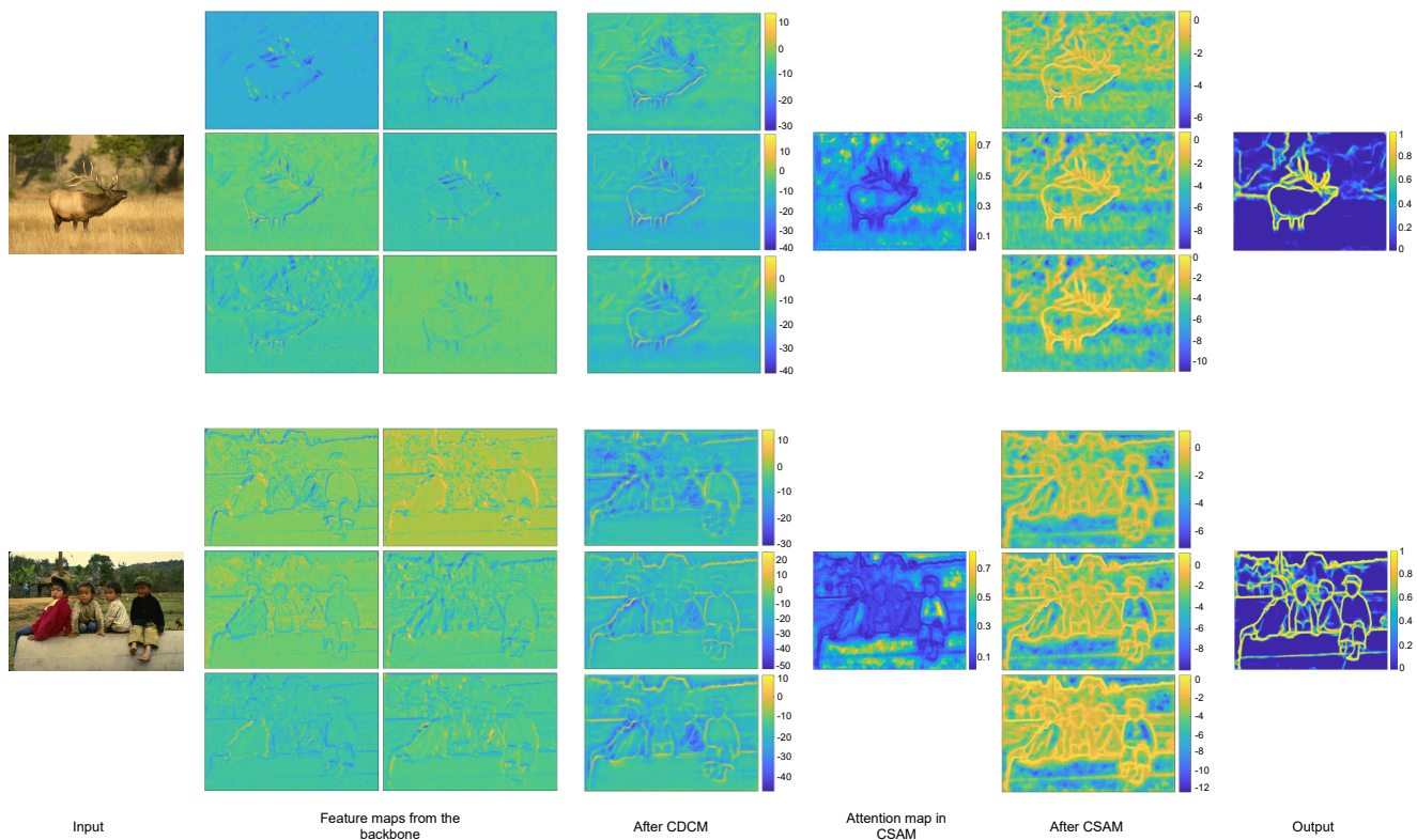
Figure 15. CDCM and CSAM can further refine the feature maps with multi-scale feature extraction and the sample adaptive spatial attention mechanism. Note that in the attention maps generated by CSAM, pixels in the background show higher intensities. This makes sense as the background pixels after CDCM have negative values, hence they will be additionally suppressed through CSAM.
