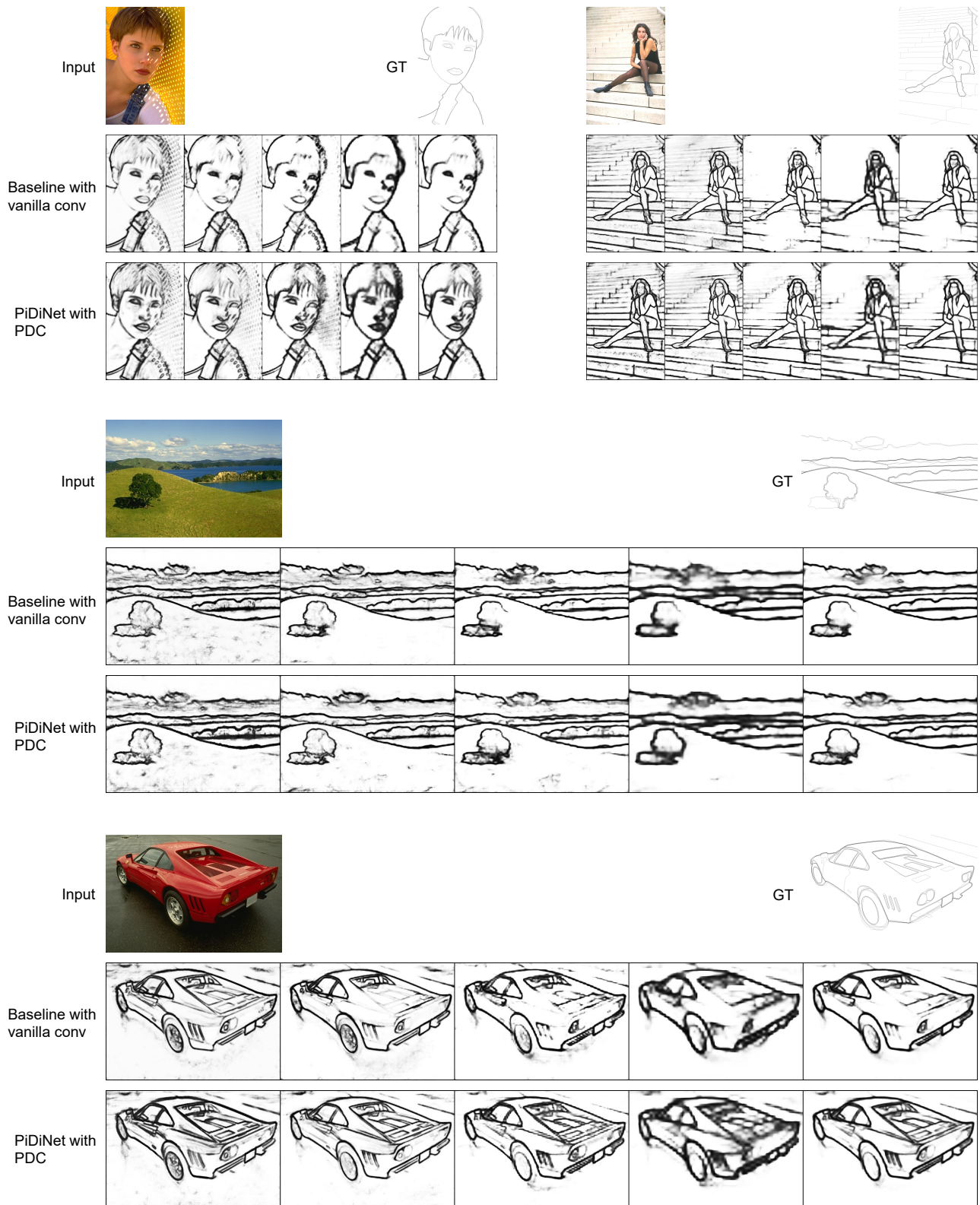
Figure 14. For each case, Top: input and ground truth image; Middle: edge maps from stage 1, 2, 3, 4 respectively and the final edge map, generated from the baseline architecture, Bottom: Corresponding edge maps generated from PiDiNet. Both the baseline architecture and PiDiNet were trained only using the BSDS500 dataset [1]. Compared with the baseline, we can see that PiDiNet can detect more useful boundaries (e.g., bangs, stairs, the contour of the tree, the characteristic textures of the car).
