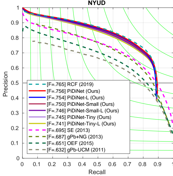
Figure 13. Precision-Recall curves of our models and some competitors on NYUD dataset.
