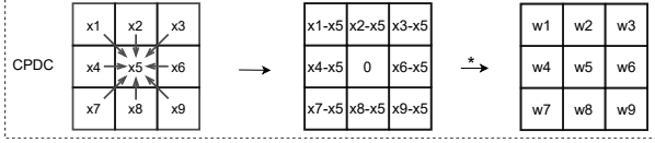
Figure 10. Selection of pixel pairs and convolution in CPDC.
