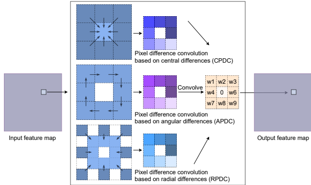
Figure 3. Three instances of pixel difference convolution derived from extended LBP descriptors [28, 30, 52]. One can derive other instances by designing the picking strategy of the pixel pairs.
